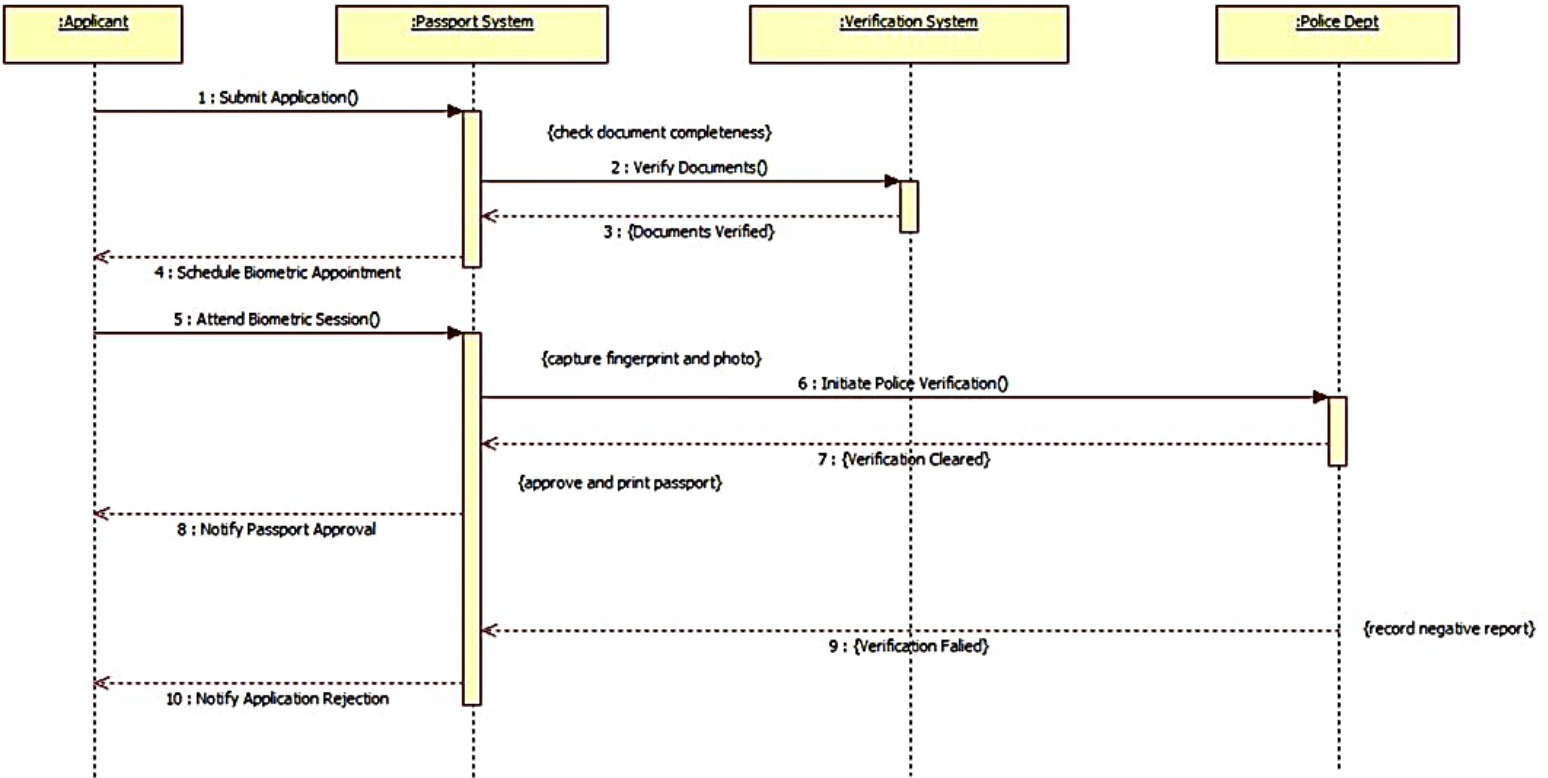
Passport Automation System Sequence Diagram
