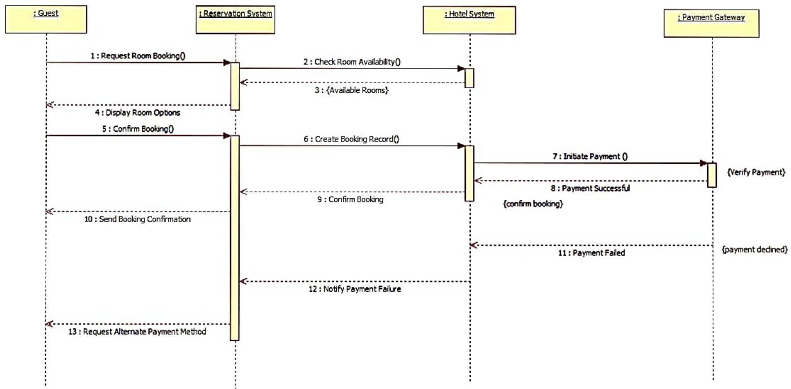
Hotel Management System Sequence Diagram
